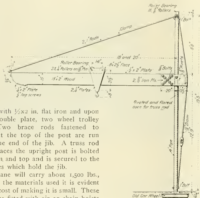
A CHEAP SHOP CRANE.
